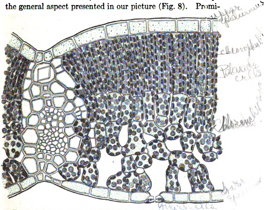
FIG. 8. — A cross section through a typical leaf, that of the European Beech; greatly magnified. The shaded round and oval grains are green in the living leaf. (Drawn, with slight changes, from a wall chart by L. Kny.)
